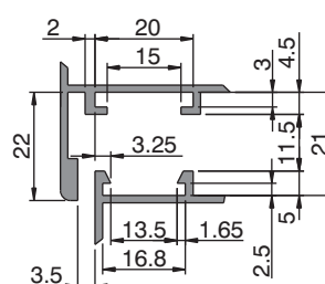
SECTION TYPE 2
