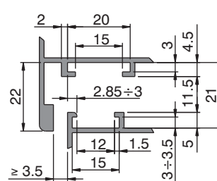
SECTION TYPE 4
