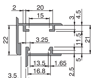
SECTION TYPE 2
