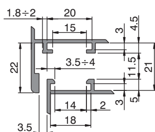
SECTION TYPE 1
