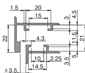
SECTION TYPE 3
