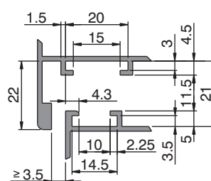
SECTION TYPE 3
