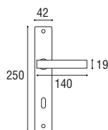
Cod. 183 CS 01 RQ Maniglia con placca \varnothing 8 x 90 Door handle with plate \varnothing 8 x 90
