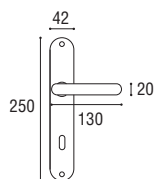
Cod. 10 CC 01 Maniglia con placca \varnothing 8 x 90 Door handle with plate \varnothing 8 x 90
