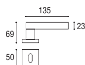
Cod. 174 CS 01 RQ Maniglia con placca \varnothing 8 x 90 Door handle with plate \varnothing 8 x 90
