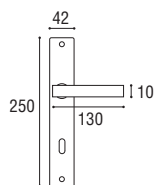
Cod. 153 CS 01 RQ Maniglia con placca \varnothing 8 x 90 Door handle with plate \varnothing 8 x 90
