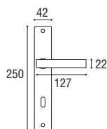
Cod. 165 CC 01 RQ Maniglia con placca \varnothing 8 x 90 Door handle with plate \varnothing 8 x 90
