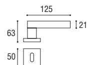
Cod. 175 CS 01 RQ Maniglia con placca \varnothing 8 x 90 Door handle with plate \varnothing 8 x 90
