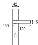
Cod. 01 CC 01 RQ Maniglia con placca \varnothing 8 x 90 Door handle with plate \varnothing 8 x 90
