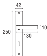
Cod. 140 CS 01 RQ Maniglia con placca \varnothing 8 x 90 Door handle with plate \varnothing 8 x 90
