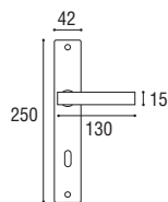
Cod. 127 CC 01 RQ Maniglia con placca \varnothing 8 x 90 Door handle with plate \varnothing 8 x 90
