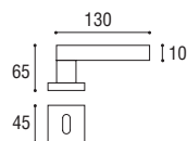
Cod. 140 CS 01 RQ Maniglia con placca \varnothing 8 x 90 Door handle with plate \varnothing 8 x 90
