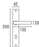
Cod. 177 CC 01 RQ Maniglia con placca \varnothing 8 x 90 Door handle with plate \varnothing 8 x 90
