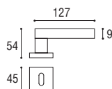
Cod. 165 CC 01 RQ Maniglia con placca \varnothing 8 x 90 Door handle with plate \varnothing 8 x 90
