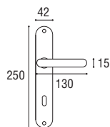
Cod. 03 CS 01 Maniglia con placca \varnothing 8 x 90 Door handle with plate \varnothing 8 x 90
