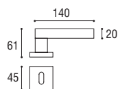
Cod. 178 CC 01 RQ Maniglia con placca \varnothing 8 x 90 Door handle with plate \varnothing 8 x 90
