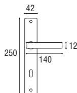
Cod. 178 CC 01 RQ Maniglia con placca \varnothing 8 x 90 Door handle with plate \varnothing 8 x 90
