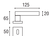
Cod. 166 CS 01 RQ Maniglia con placca \varnothing 8 x 90 Door handle with plate \varnothing 8 x 90
