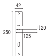
Cod. 175 CS 01 RQ Maniglia con placca \varnothing 8 x 90 Door handle with plate \varnothing 8 x 90
