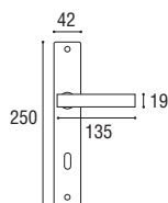
Cod. 174 CS 01 RQ Maniglia con placca \varnothing 8 x 90 Door handle with plate \varnothing 8 x 90
