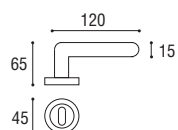
Cod. 152 CS 01 Maniglia con placca \varnothing 8 x 90 Door handle with plate \varnothing 8 x 90
