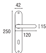
Cod. 152 CS 01 Maniglia con placca \varnothing 8 x 90 Door handle with plate \varnothing 8 x 90
