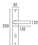
Cod. 180 CS 01 RQ Maniglia con placca \varnothing 8 x 90 Door handle with plate \varnothing 8 x 90
