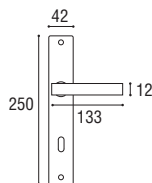
Cod. 186 CC 01 RQ Maniglia con placca \varnothing 8 x 90 Door handle with plate \varnothing 8 x 90
