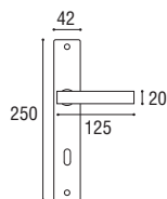
Cod. 166 CS 01 RQ Maniglia con placca \varnothing 8 x 90 Door handle with plate \varnothing 8 x 90
