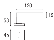
Cod. 01 CC 01 RQ Maniglia con placca \varnothing 8 x 90 Door handle with plate \varnothing 8 x 90
