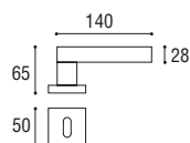
Cod. 183 CS 01 RQ Maniglia con placca \varnothing 8 x 90 Door handle with plate \varnothing 8 x 90
