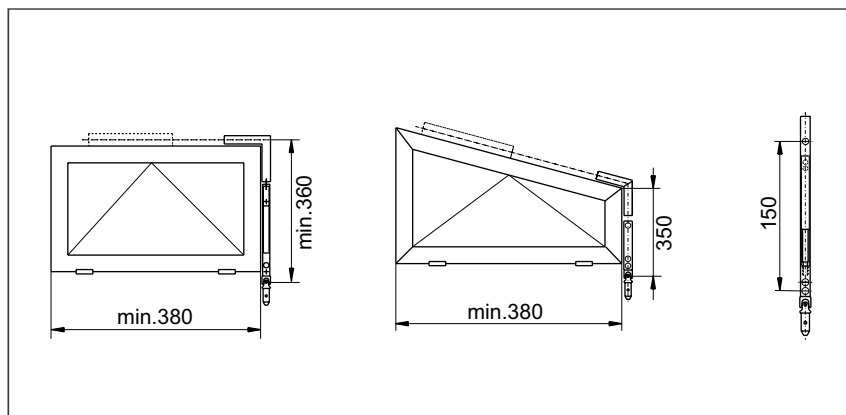
Rectangular and angular windows with GEZE Fz 91
