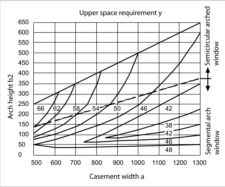
D dimension and upper space requirement for semicircular and segmental arch windows
