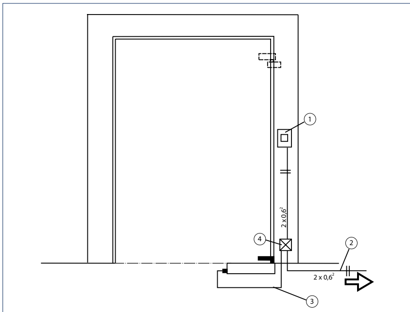
Electrical installation TS 550 E / TS 550 E-G:
