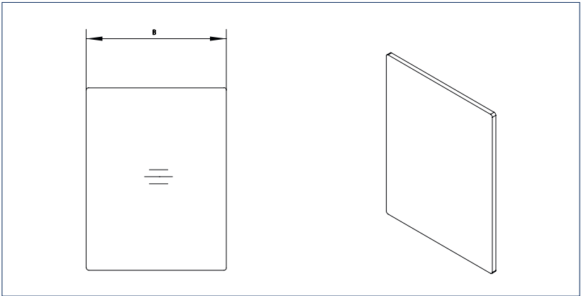
End cover caps profile design 40, glass thicknesses 8, 10 and 12 mm B = Width (30 mm for glass thicknesses 8 and 10 mm, 32 mm for glass thickness 12 mm)
