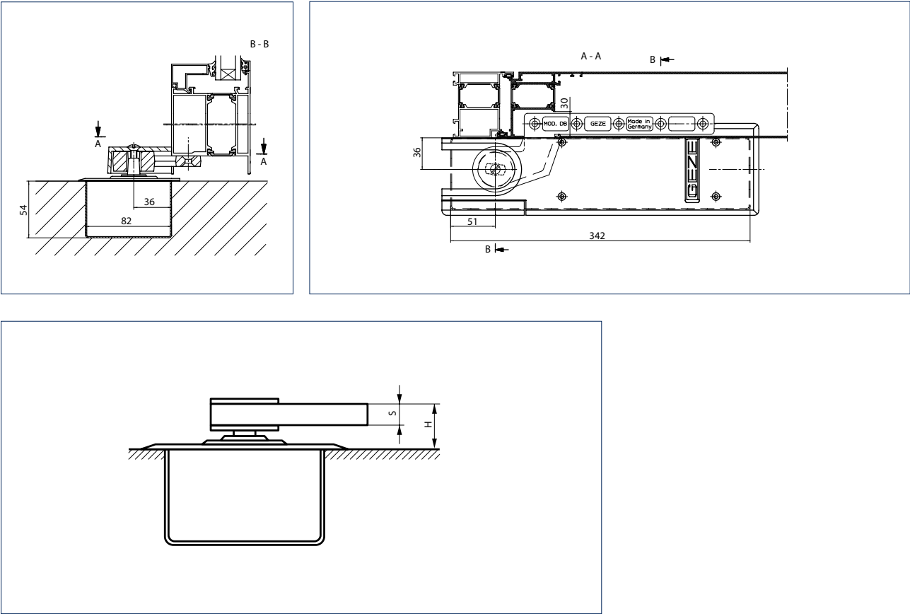
Door rail model DM, DB, EK, FK for single-action doors H = Installation height dimension
