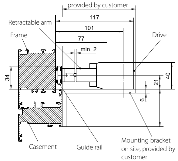
Head point detail
