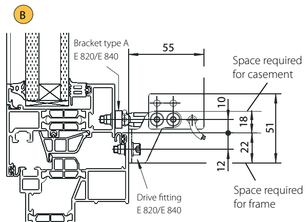
Fitting dimensions drive fitting type A with bracket type A
