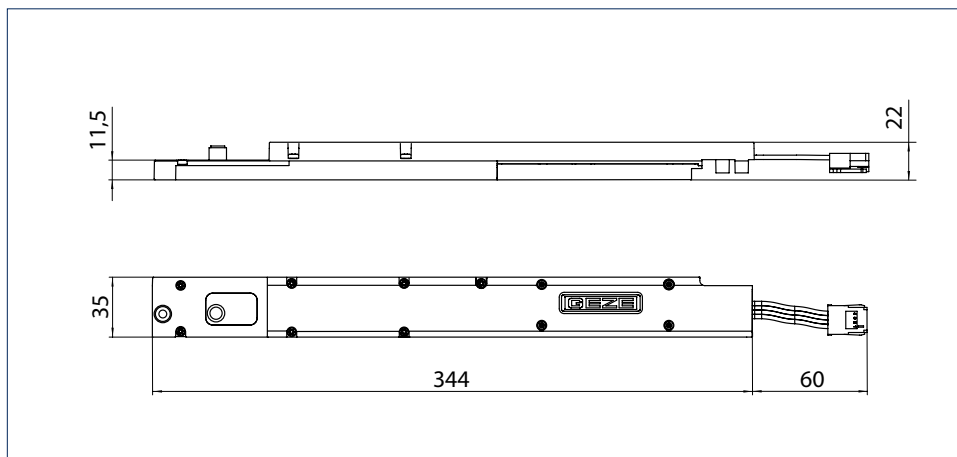
Main dimensions E 905, E 906 mirrored
