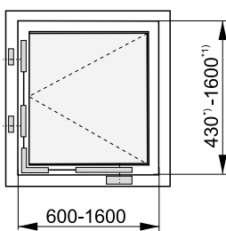
Side hung windows
