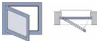
Side hung casement, inward opening
