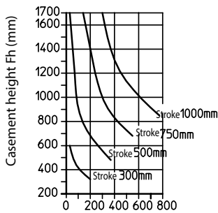
Space required for swivel movement (mm)
