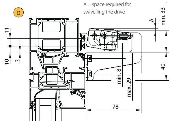
Fitting dimensions drive fitting type B with bracket type B
