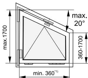
Angular windows Bottom hung
