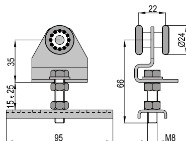
Fix trolley with 2 wheels.
