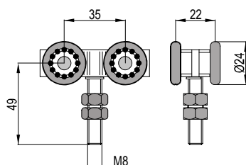
Rotating trolley in aluminium with 4 wheels.
