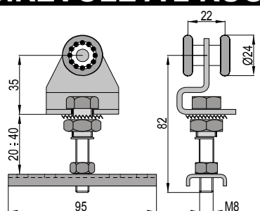
Rotating trolley with 2 wheels.
