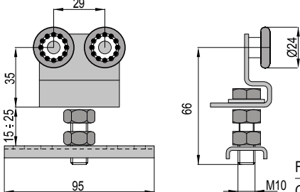
Fix trolley with 2 wheels. Chariot fixe à 2 roulements.
