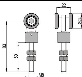
Rotating trolley with 2 wheels.
