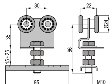
Fix trolley with 4 wheels.
