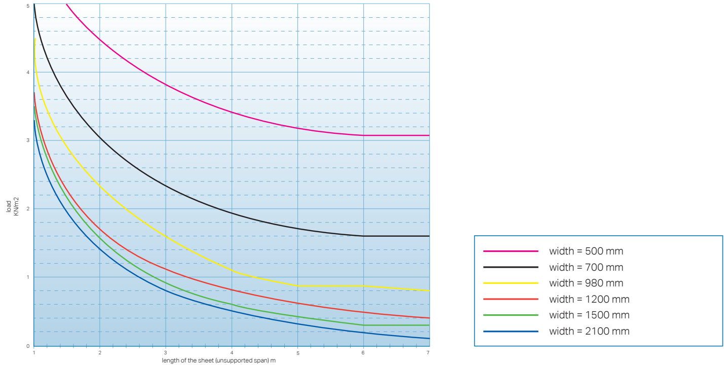
load bearing characteristics of Makrolon multi UV 7/20-14 flat glazed
