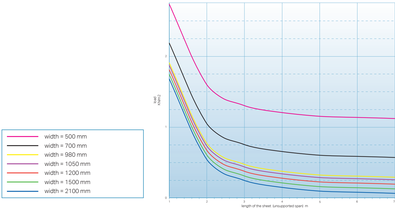
load bearing characteristics of Makrolon multi UV 4/10-6 flat glazed
