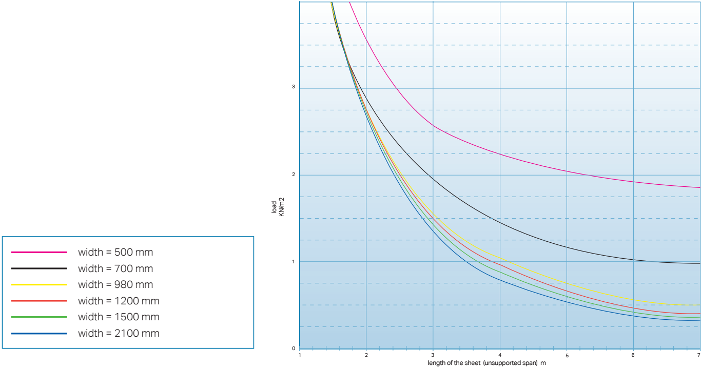
load bearing characteristics of Makrolon multi UV 5X/16-25 flat glazed
