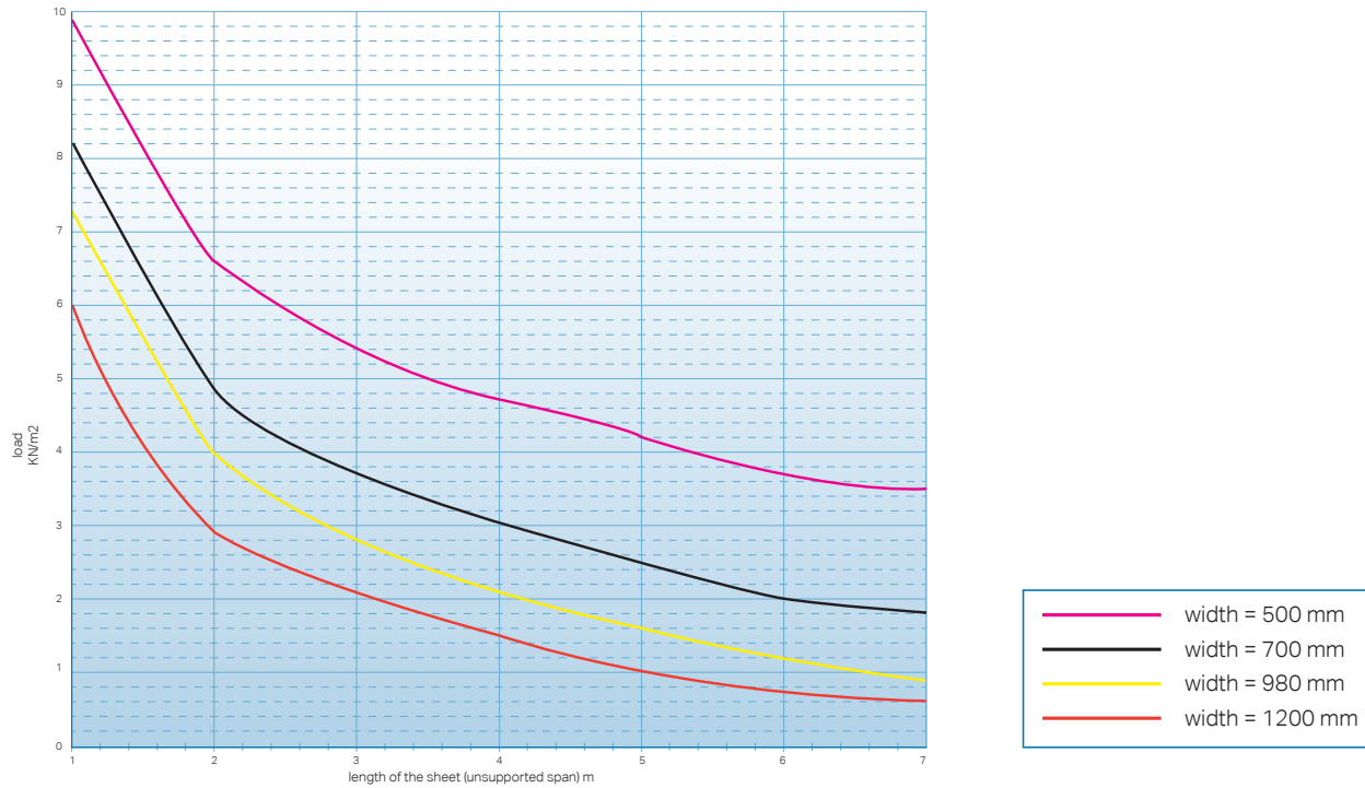
load bearing characteristics of Makrolon multi UV 7M/32-28 flat glazed
