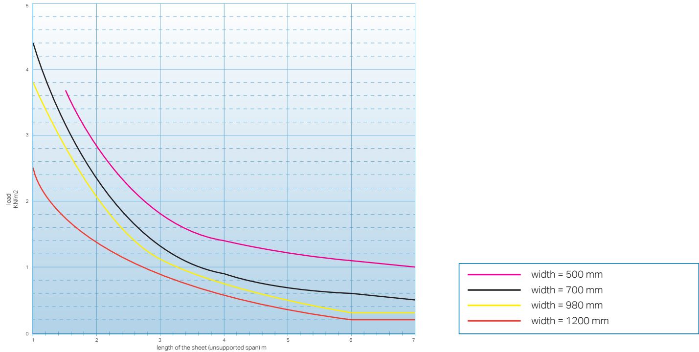
load bearing characteristics of Makrolon multi UV 7M/20-28 flat glazed
