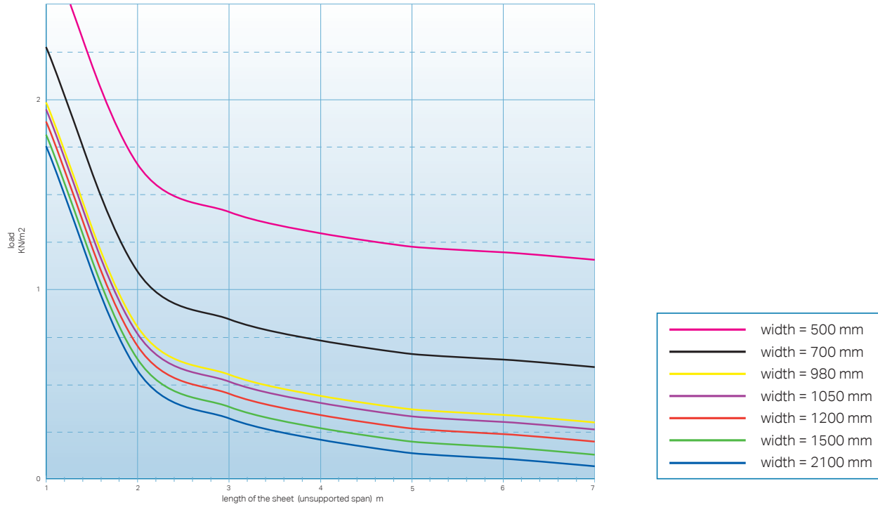
load bearing characteristics of Makrolon multi UV 2/10-10.5 flat glazed
