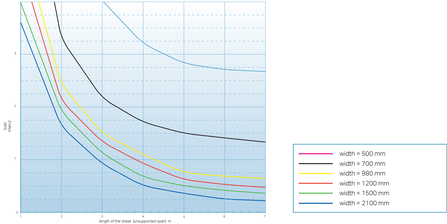
load bearing characteristics of Makrolon multi UV 3/16-20 flat glazed
