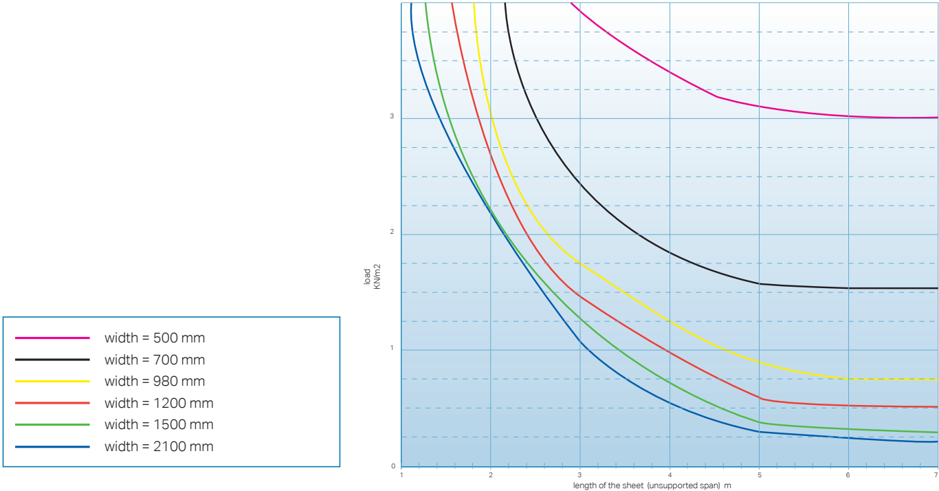
load bearing characteristics of Makrolon multi UV 5M/25-20 flat glazed
