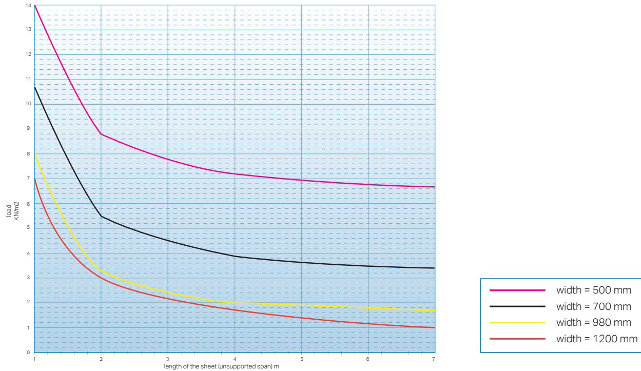
load bearing characteristics of Makrolon multi UV 7M/50-28 flat glazed
