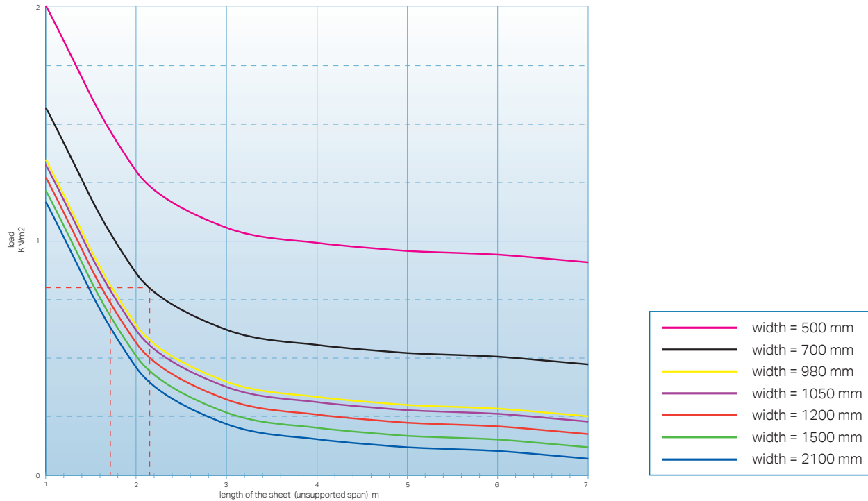
load bearing characteristics of Makrolon multi UV 2/6-8 flat glazed
