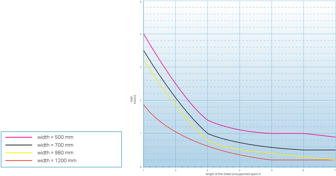
load bearing characteristics of Makrolon multi UV 7M/16-28 flat glazed
