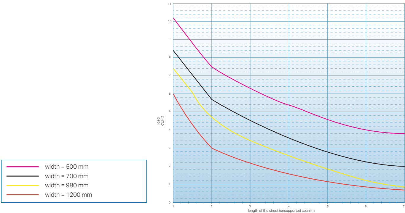
load bearing characteristics of Makrolon multi UV 7M/40-28 flat glazed
