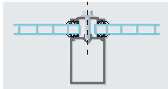
Profile system with preset clamping pressure.
