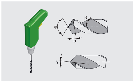
Drills for Makrolon® sheets
