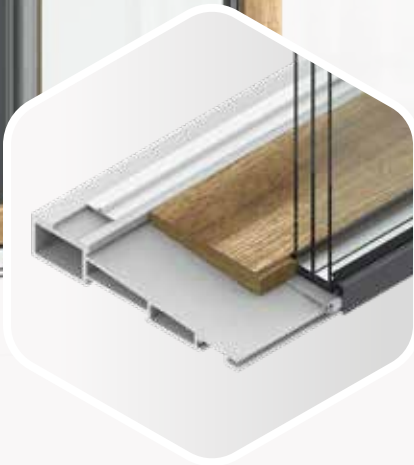
THRESHOLD CONSTRUCTION with fixed glazing
