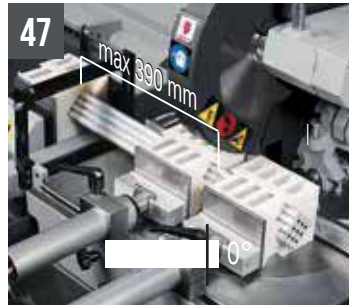
47 COBRA 352 NC 5.0 - set of comb jaws in teflon for bundle cutting (max mm 75x75 - min 20x20)
