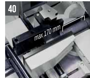
TIGER 352 NC 5.0 Special vice to reduce restpiece
