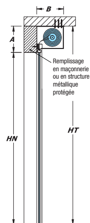
In-reveal mounting
