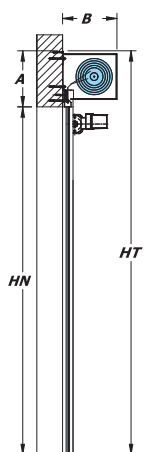
Front mounting
