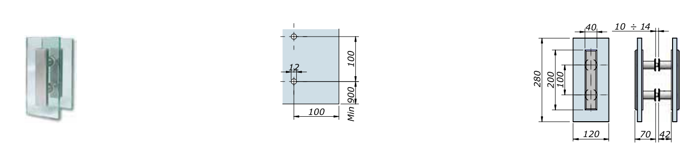
Maniglia in vetro Glass handle
