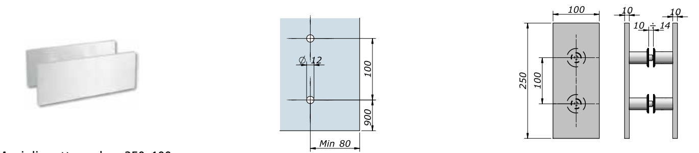
Maniglia rettangolare 250x100 mm Rectangular handle 250x100 mm
