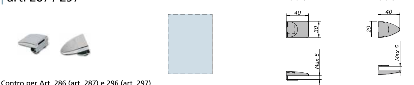
Contro per Art. 286 (art. 287) e 296 (art. 297) Lock keeper for Art. 286 (art. 287) and 296 (art. 297)
